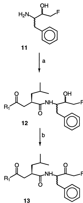
Scheme 3. Reagents: (a) NMM, IBCF, 5d , \text{CH}_2\text{Cl}_2 , -20 to 23^\circ\text{C} or BOP, HOBT, NMM, DMF, 0 – 23^\circ\text{C} ; (b) Dess–Martin periodinane, \text{CH}_2\text{Cl}_2 , 23^\circ\text{C} .
