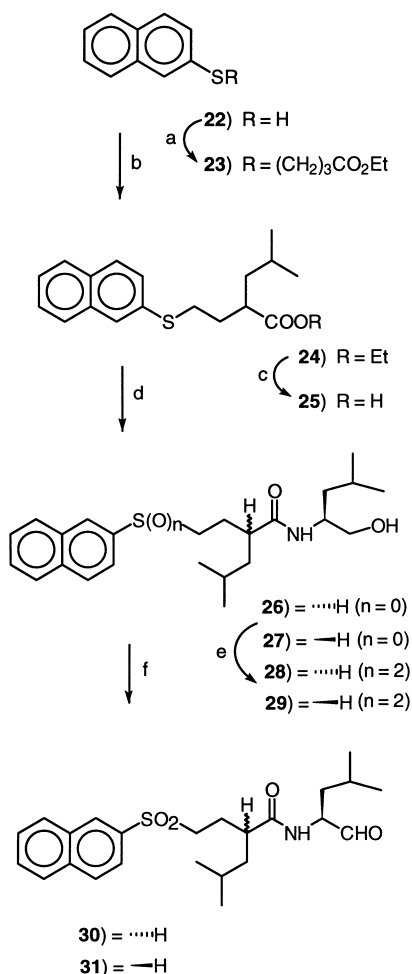
Scheme 5. Reagents: (a) 60% NaH, Br(CH 2 ) 3 COOEt, THF, 0–23 °C; (b) LDA, 1-iodo-2-methylpropane, THF-hexane-HMPA, –78 °C to 23 °C; (c) LiOH·H 2 O, EtOH-H 2 O, reflux; (d) ( S )-leucinol, BOP, HOBT, NMM, DMF, 0–23 °C; (e) m -CPBA, CH 2 Cl 2 , 0–23 °C; (f) Pyr·SO 3 , Et 3 N, DMSO-CH 2 Cl 2 , 0–23 °C.
