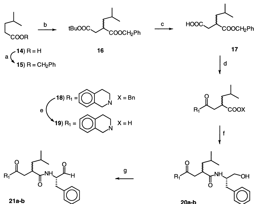
Scheme 4. Reagents: (a) Benzyl alcohol, p -toluenesulfonic acid monohydrate, benzene, reflux (Dean–Stark); (b) LDA, t -butyl bromoacetate, THF–hexane–HMPA, -78^{\circ}\text{C} to 0^{\circ}\text{C} ; (c) 90% TFA, CH 2 Cl 2 , 23^{\circ}\text{C} ; (d) 1,2,3,4-tetrahydroisoquinoline, BOP-Cl, Et 3 N, CH 2 Cl 2 , 23^{\circ}\text{C} ; (e) H 2 , 10% Pd–C (Degussa, H 2 O content 50%), MeOH; (f) BOP, HOBT, NMM, DMF, 0 – 23^{\circ}\text{C} ; (g) Pyr.SO 3 , Et 3 N, DMSO–CH 2 Cl 2 , 0 – 23^{\circ}\text{C} .
