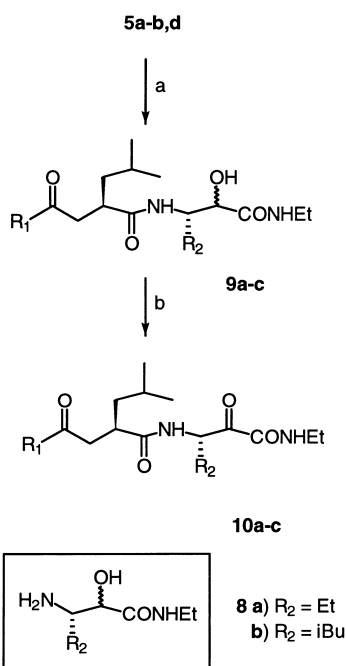
Scheme 2. Reagents: (a) NMM, IBCF, THF-DMF, -20 to 23^\circ\text{C} or BOP, HOBT, NMM, DMF, 0 – 23^\circ\text{C} ; (b) Dess–Martin periodinane, \text{CH}_2\text{Cl}_2 , 0 – 23^\circ\text{C} .
