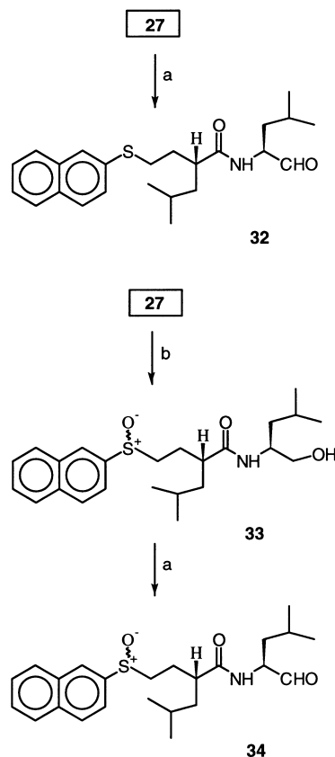
Scheme 6. Reagents: (a) Pyr·SO 3 , Et 3 N, DMSO-CH 2 Cl 2 , 0–23 °C; (b) Davis' oxaziridine (PhSO 2 N(O)CHPh), CH 2 Cl 2 , 23 °C.
