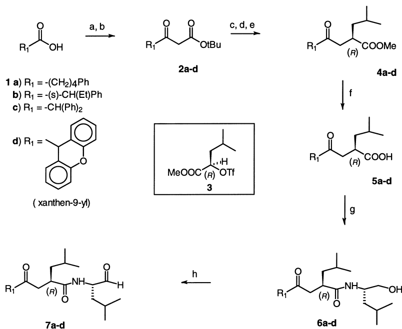
Scheme 1. Reagents: (a) 1,1'-carbonyldiimidazole, THF, 0–23 °C; (b) Li + -CH 2 COOtBu, THF; -78 °C to 0 °C; (c) 60% NaH, THF, 3, 23 °C; (d) TFA, 23 °C; (e) C 6 H 6 , reflux; (f) LiOH, MeOH-H 2 O; 70–75 °C; (g) ( S )-leucinol, BOP, HOBT, NMM, DMF 0–23 °C; (h) Pyr.SO 3 , Et 3 N, DMSO-CH 2 Cl 2 , 0–23 °C.
